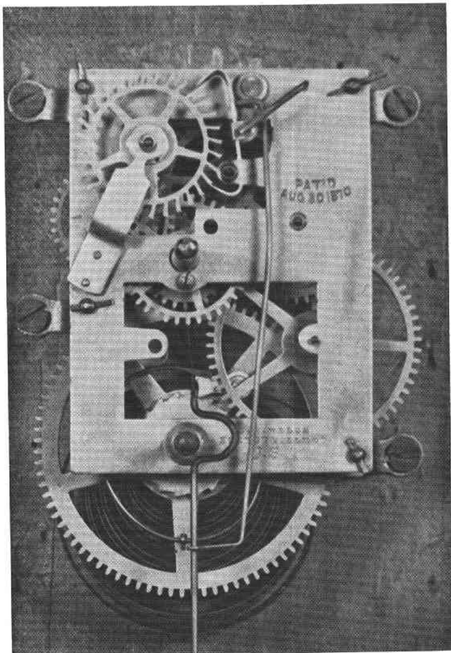
Fig. 45 Eight-day Movement of Figure 44
