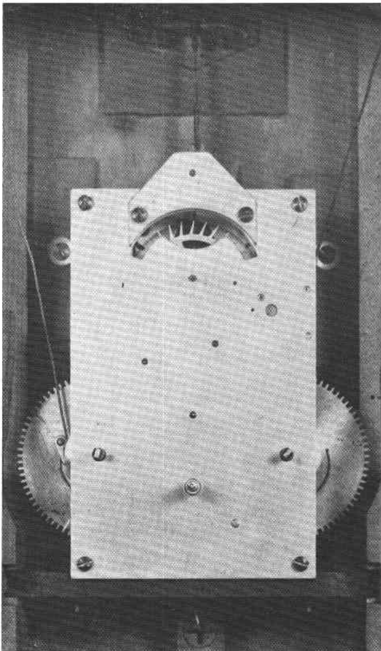
Fig. 39 Eight-day Movement of Figure 38
