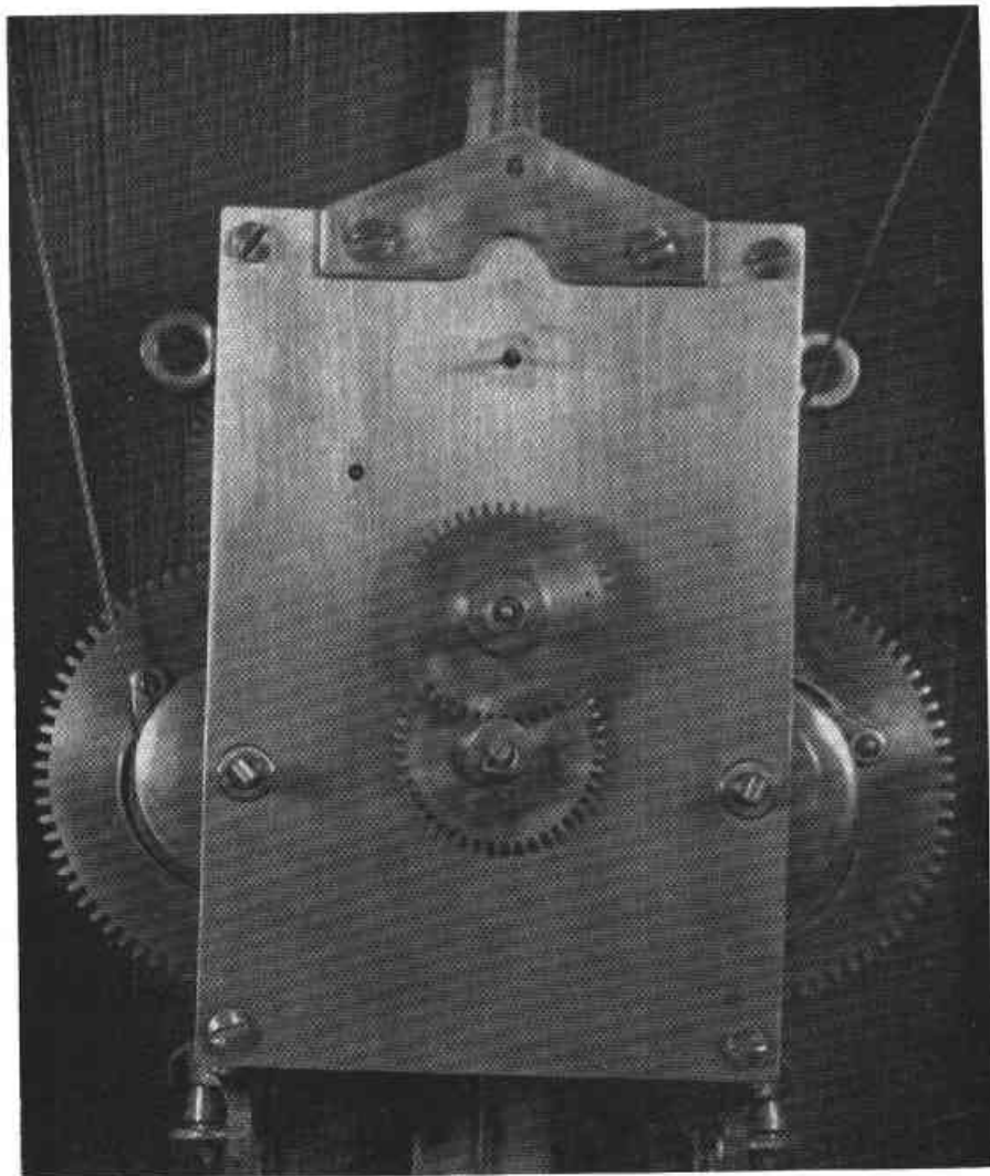
Fig. 43 Eight-day Movement of Figure 42
